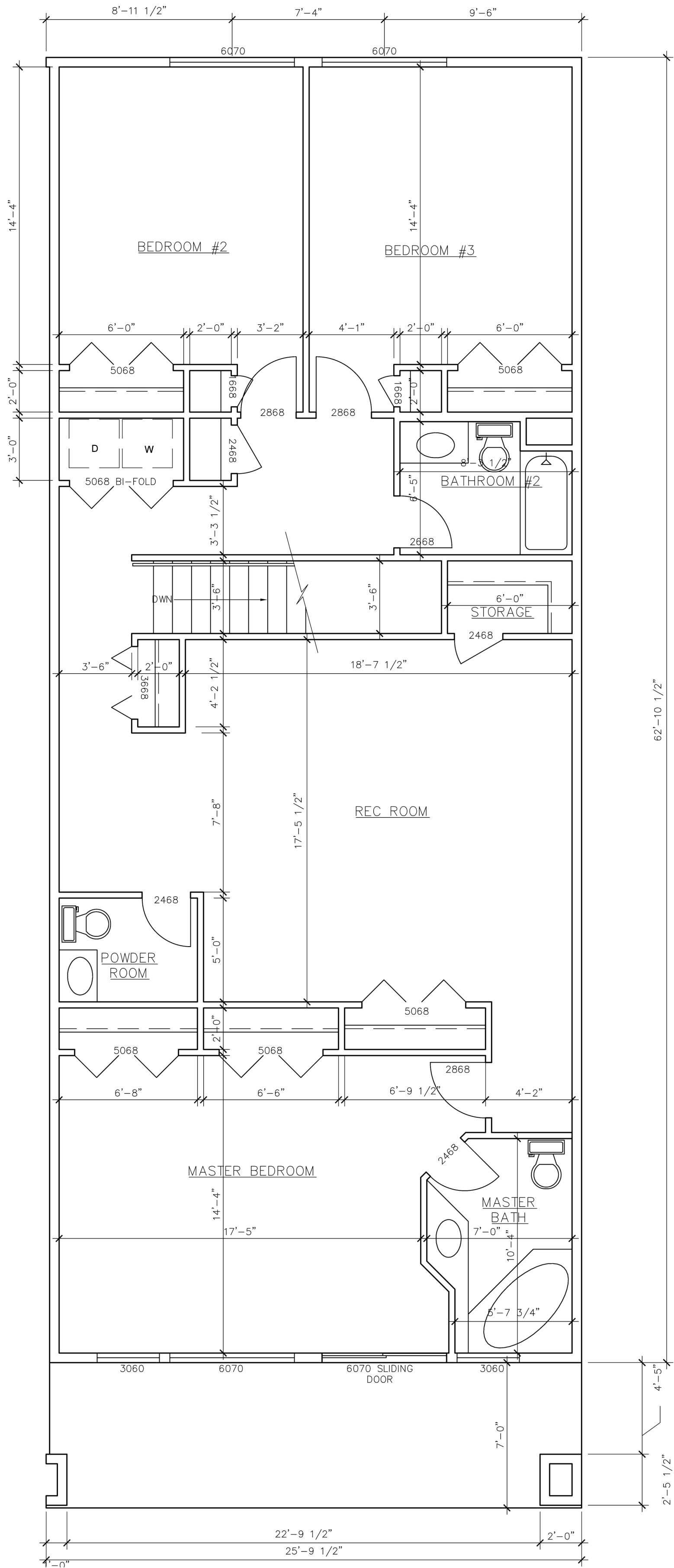
BLUE UPPER FLOOR PLAN (OPTION 2)
