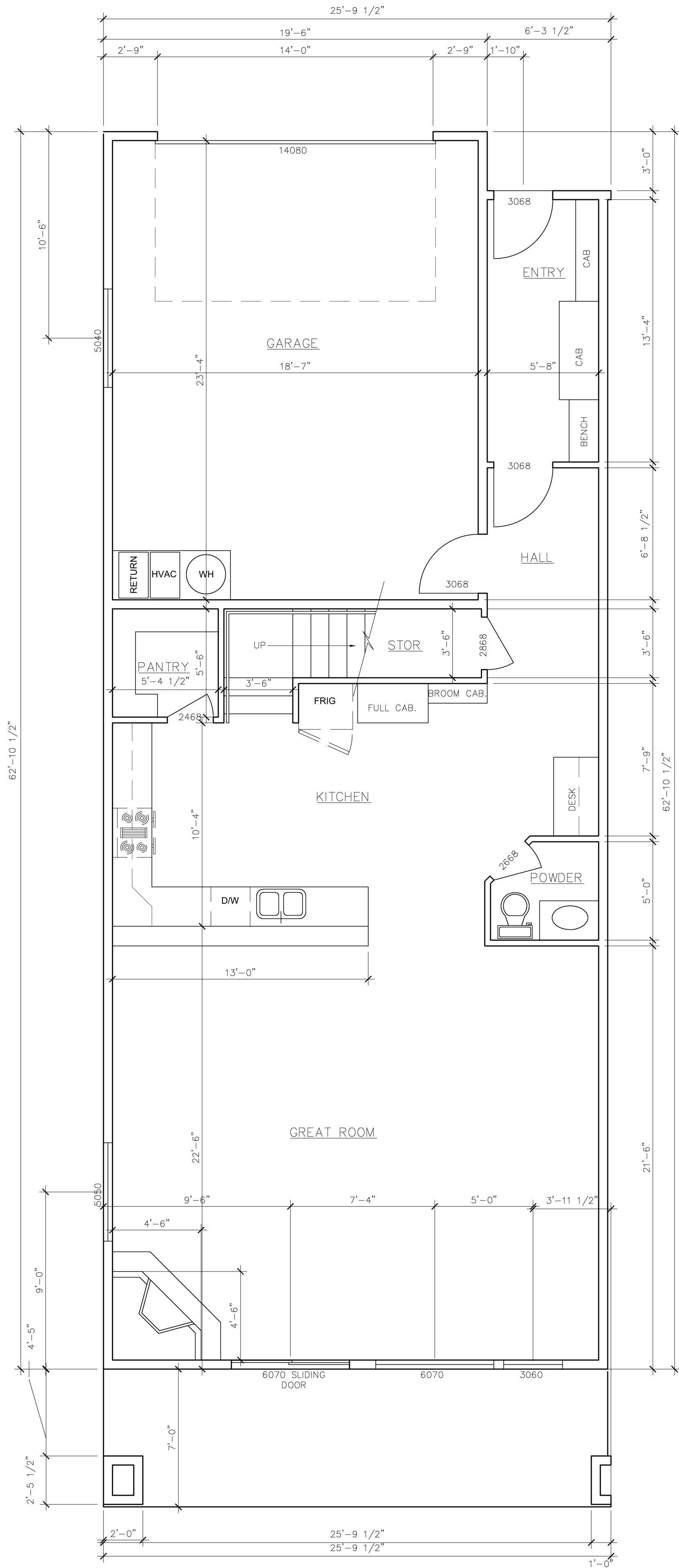
BLUE MAIN FLOOR PLAN
